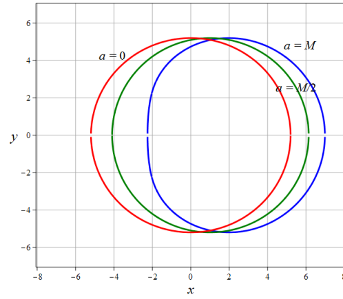
Fig. 14. Contour of the shadow of a rotating collapsar in the standard Kerr metric with M = \text{const} , a = (0; 0.5; 1)M_{ir} .
