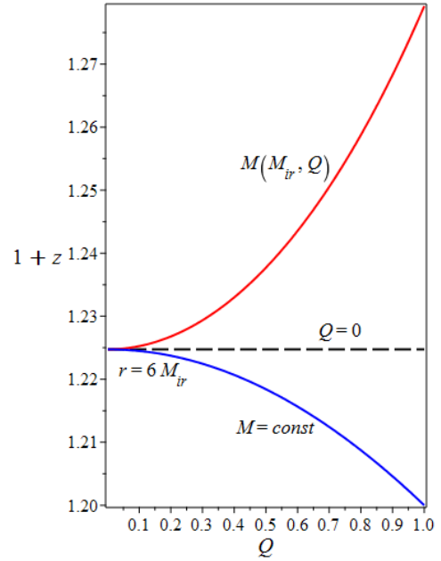
Fig. 1. Dependence on Q of time dilation, Fig. 2. Dependence on Q of redshift, r = 6M_{ir} . r = 6M_{ir} .
