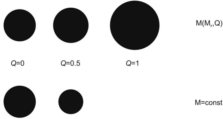
Fig. 5. Charge dependence of the shadow of a charged collapsar in two approaches.
