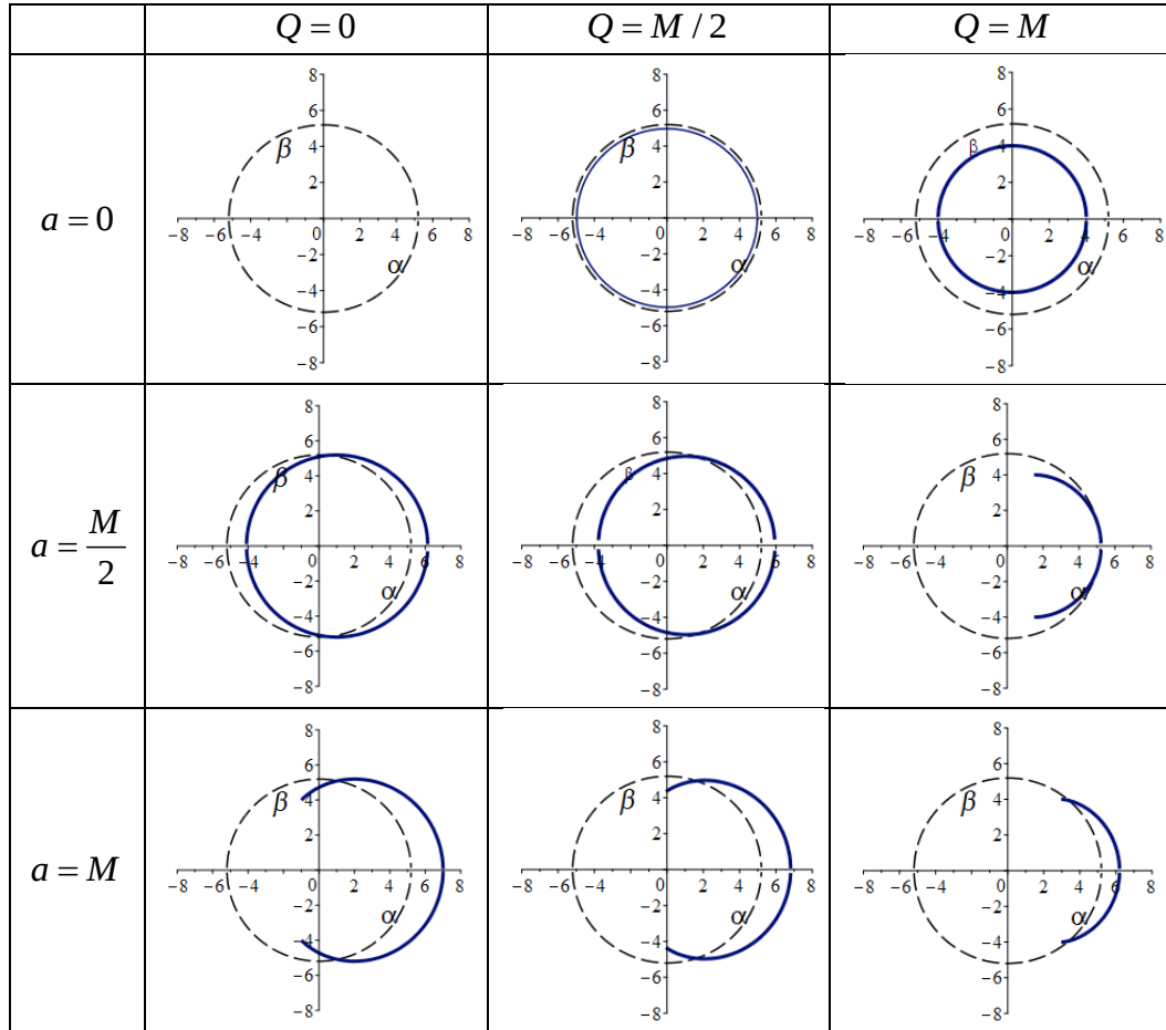
Fig. 1. The contour of the shadow of a compact source in the standard form of the Kerr-Newman metric (1) at the condition M = \text{const} = 1 in (6)-(7) ( \theta = \pi / 2 ) (see [7]).
