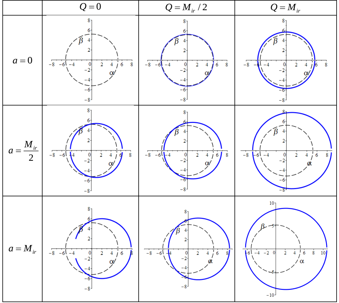
Fig. 2. Shadow contour of a compact source in the Kerr-Newman metric with irreducible mass (4), when (3) inserted into (6)-(7) and the condition M_{ir} = \text{const} = 1 is used ( \theta = \pi / 2 ) (see [6]).
