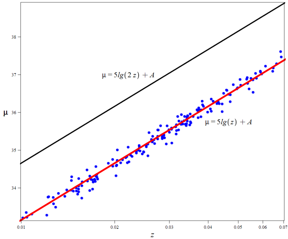
Fig. 1. Graph "distance modulus - redshift" for SN 1a in the linear part (in the logarithmic scale of z ), A = 5\lg(c / H_0) + 25 , H_0 = 70 \text{ km / sec} \cdot \text{Mpc} , the data from [10a]. Black line – the double redshift with shift \delta\mu = 5\lg(2) = 1.5 .
