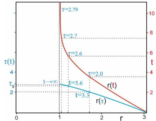
Fig. 1. The worldline of a falling test particle in terms of world time t and proper time \tau .
