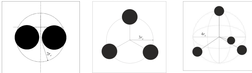
Fig. 5. Gravitational freezing of two, three and four frozars of the same mass on gravitational radius of the center of inertia of the system nr_g ( n = 2, 3, 4 ).
