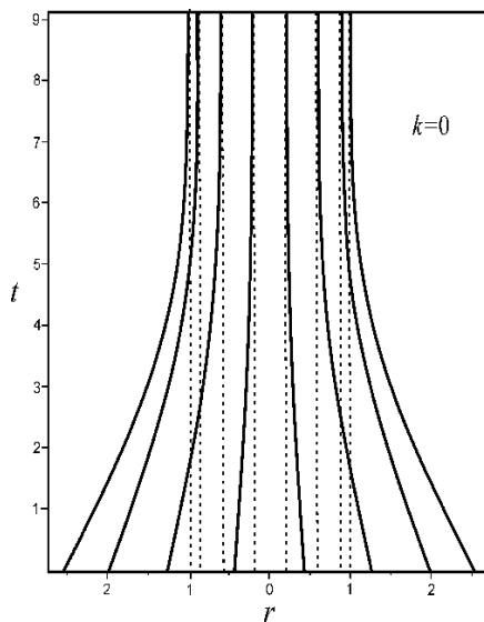
Fig. 2. World lines of stellar particles along the diameter (in units of the gravitational radius) according to the OS solution. At large t , particles on the surface freeze outside the gravitational radius, and the inner layers freeze near their asymptotes (dashed lines).
