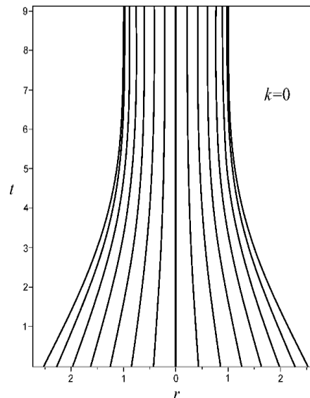
Fig. 3. OS worldlines from Fig. 2 with a slightly more number of layers to show how different layers freeze.
