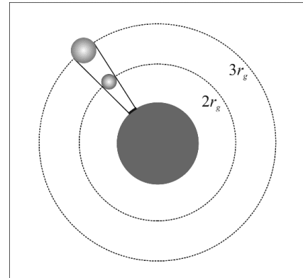
Fig. 4. The radial fall of a neutron star of the mass 1.5M_{\odot} onto the frozar of mass 7M_{\odot} , which leads to flattening of the neutron star (like a mascon on the Moon) and freezing on the frozar surface like a "hairstyle". This leads to local inhomogeneity of the frozar field and its shadow.
